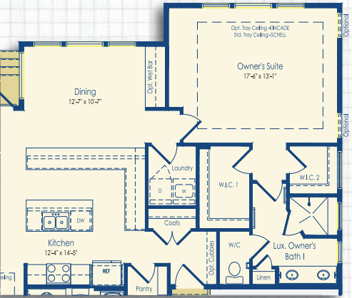
Optional Luxury Owner's Suite I
