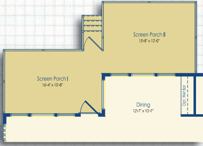
Optional Screen Porch I and Optional Screen Porch II
