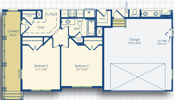
Optional Elevation B Front Porch
