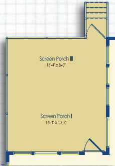
Optional Screen Porch I and Screen Porch III
