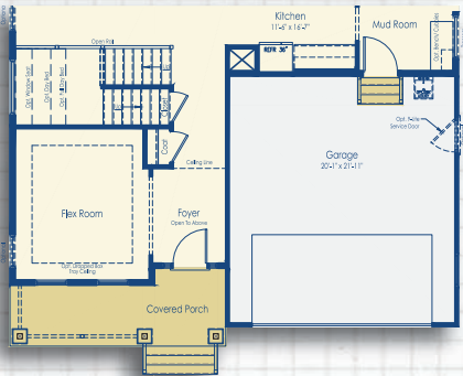
First Floor Craftsman Elevation
