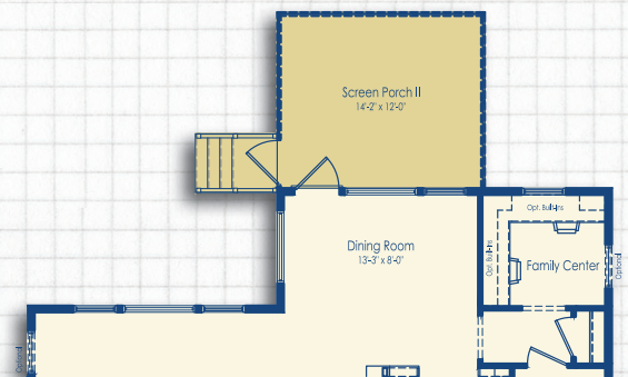
Optional Screen Porch II
