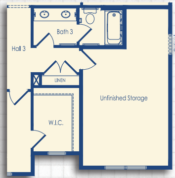
Optional Bath 3 with 4' Garage Extension
