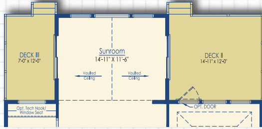
Optional Sunroom with Optional Decks II & III
