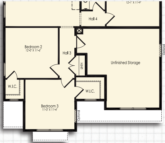
Included Elevation A and Optional Modern Farmhouse Second Floor
