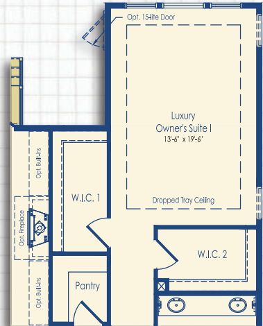
Optional Luxury Owner's Suite I with 2ft Rear Extension
