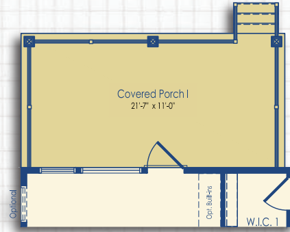
Optional Covered Porch I
