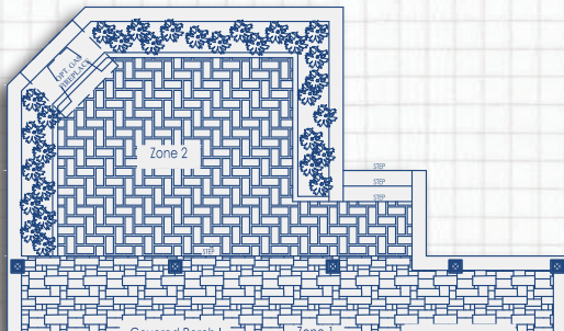
Optional Courtyard with Covered Porch I and Covered Porch II
