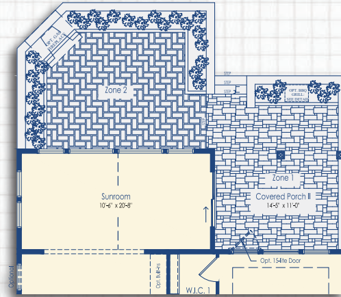
Optional Courtyard with Sunroom and Covered Porch II
