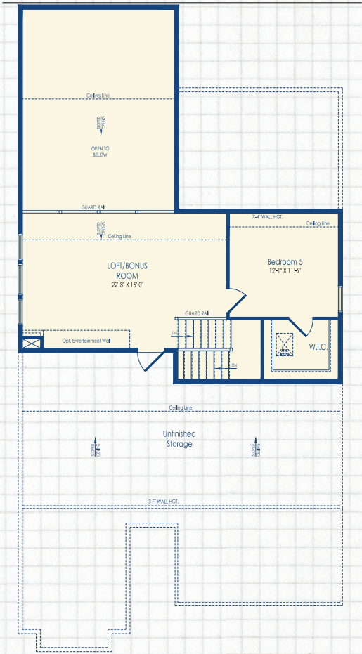
Optional Second Floor with Bedroom 5
