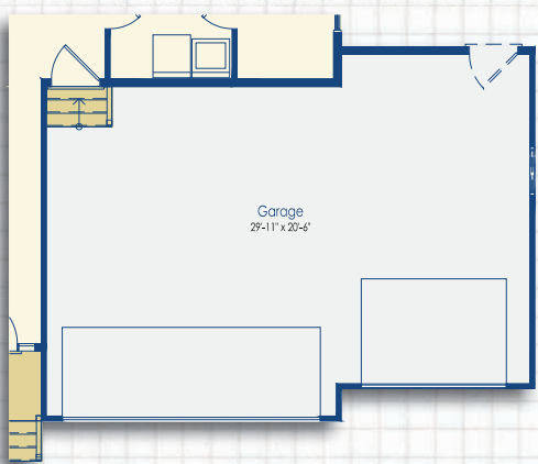
Optional 3-Car Garage Elevation B
