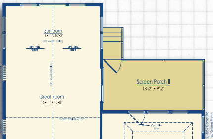
Optional Sunroom with Screen Porch II
