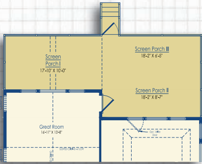
Optional Screen Porch I, II, and II
