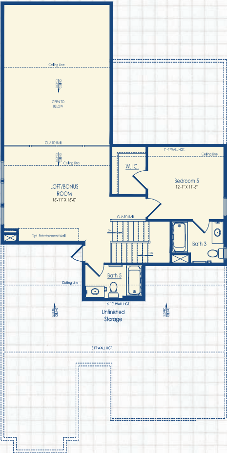
Optional Second Floor with Bedroom 6 with Bath 3
