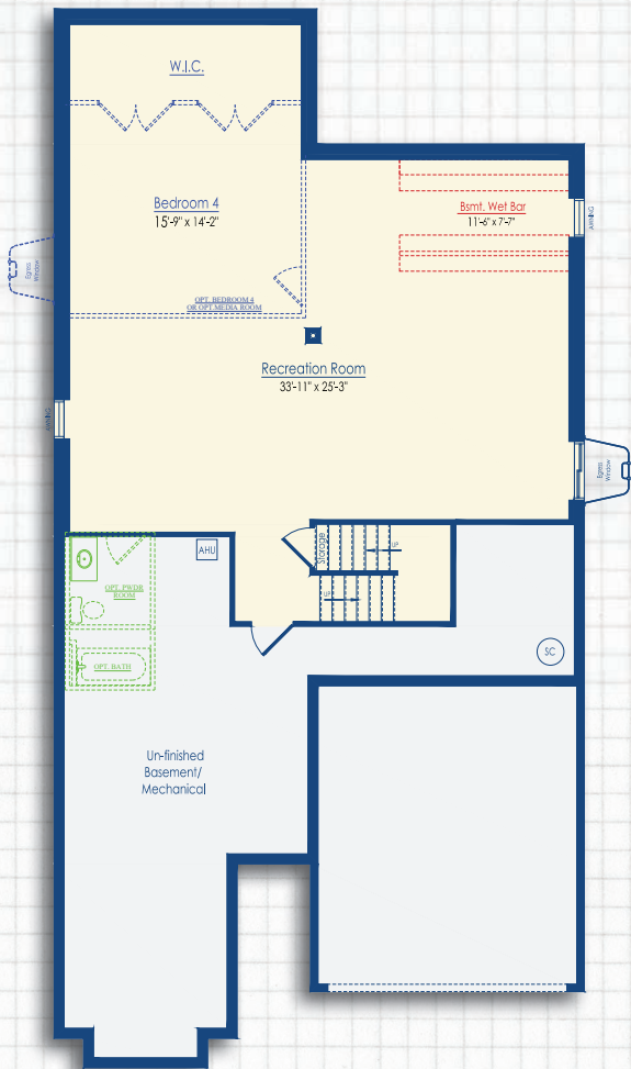
Optional Finished Basement Schell Style A, B and Farmhouse Style
