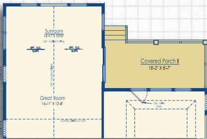
Optional Sunroom with Covered Porch II
