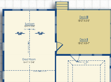
Optional Sunroom with Decks II and III with Luxury Owner’s Suite I or II
