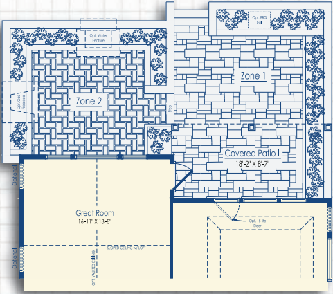
Optional Courtyard with Luxury Owner's Suite I or II and Covered Patio
