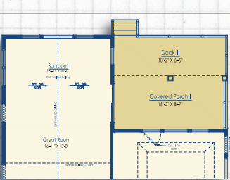
Optional Sunroom with Covered Porch II and Deck III with Luxury Owner’s Suite I or II
