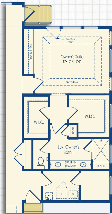
Optional Luxury Owner's Suite I
