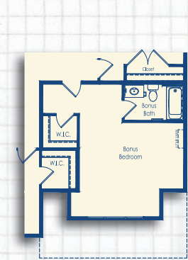
Optional Bonus Bedroom with 4' Garage Extension Craftsman Elevation
