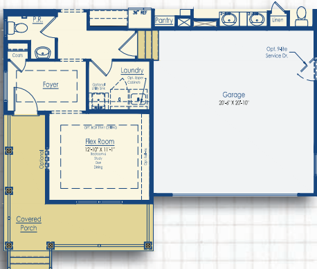
Optional Elevation C First Floor
