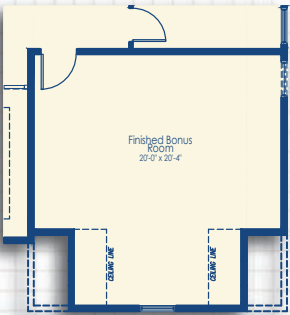
Second Floor Plan with Finished Bonus Room Elevation A
