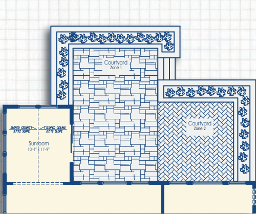
Optional Courtyard with Sunroom
