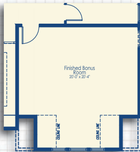
Second Floor Plan with Finished Bonus Room Craftsman Elevation
