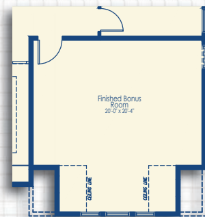
Second Floor Plan with Finished Bonus Room Craftsman Elevation
