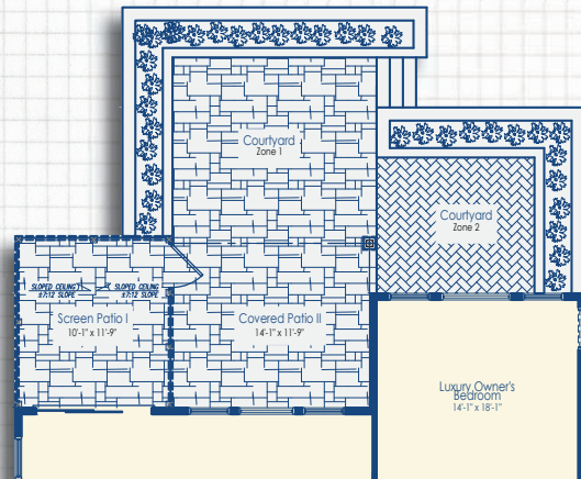
Optional Courtyard with Screen Patio I, Covered Patio II, & Luxury Owner's Suite
