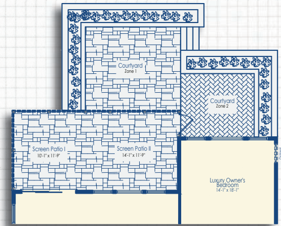
Optional Courtyard with Screen Patio I & II and Luxury Owner's Suite
