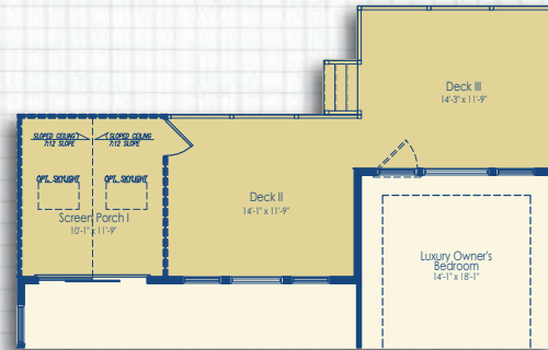
Optional Screen Porch I with Deck II & III and Luxury Owner's Suite
