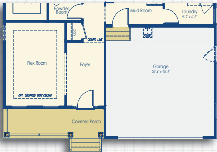
First Floor Southern Elevation
