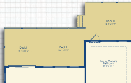
Optional Deck I, II, & III with Luxury Owner's Suite
