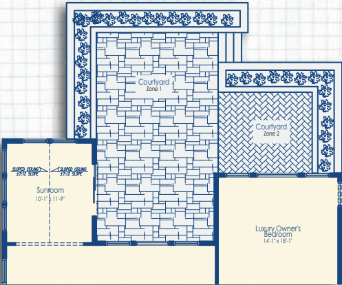
Optional Coutryard with Sunroom and Luxury Owner's Suite
