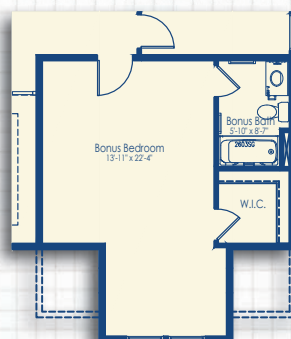
Bonus Bedroom with Bath Modern Farmhouse Elevation
