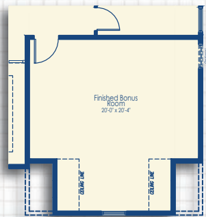
Second Floor Plan with Finished Bonus Room Elevation A
