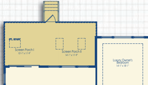
Optional Screen Porch I & II with Luxury Owner's Suite
