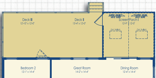
Optional Screen Porch I &amp; Deck II &amp; III
