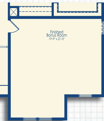
Finished Bonus Room Modern Farmhouse
