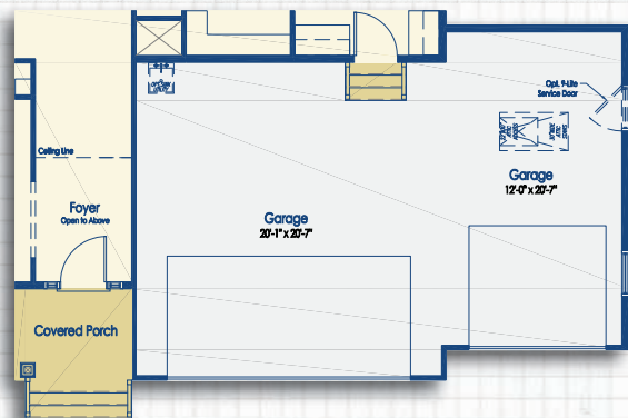
Optional 4' Garage Extension Elevation B, C, & Modern Farmhouse
