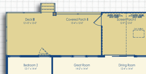
Optional Screen Porch I with Covered Porch II & Deck III
