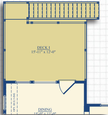
Optional Deck I Shown with Optional Stairs. Located off of the Dining Room Stair Location #3
