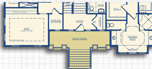
Second Floor Optional Craftsman Elevation
