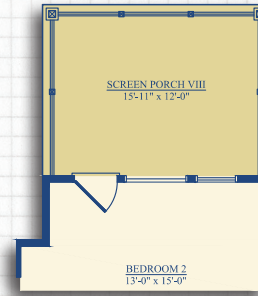
Optional Screen Porch VIII Located off of Bedroom 2
