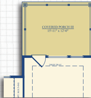
Optional Covered Porch III Located off of the Owner's Suite
