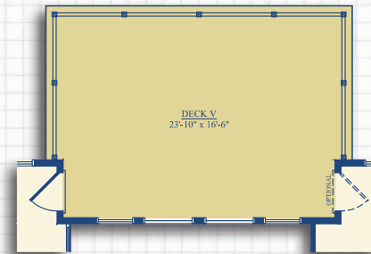
Optional Deck V Shown with Loft & Bedroom, or Second Owner's Suite. Must select Covered Porch II, Deck II, or Screen Porch V
