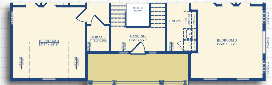
Third Floor Optional Southern Elevation
