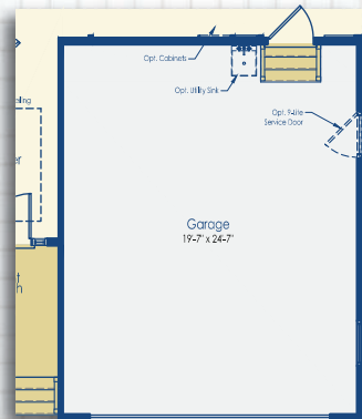
Optional 4' Garage Extension Craftsman Elevation
