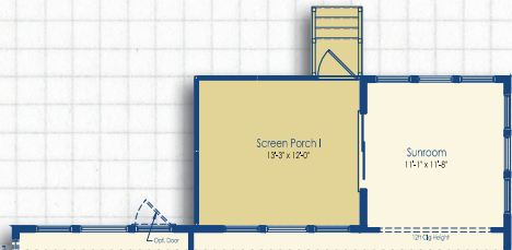
Optional Sunroom with Screen Porch I
