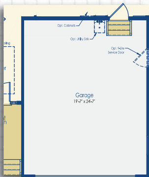
Optional 4' Garage Extension Elevation A
