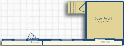
Optional Screen Porch II
