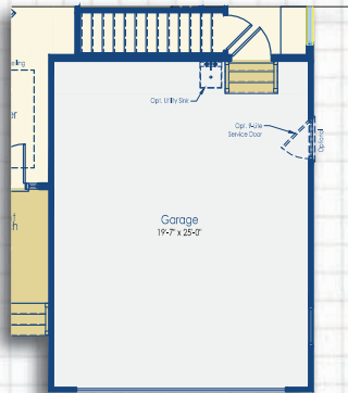
Optional 4' Garage with Basement Stairs Elevation A
