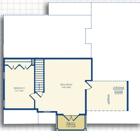
Optional Bedroom 5 with Optional Finished Bonus Room Elevation E - Also available with open rail staircase to the bonus room.
