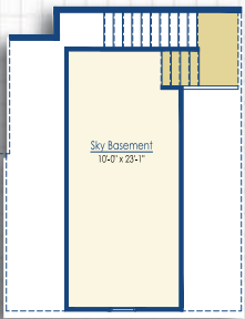
Optional Sky Basement Option may vary per elevation selected.
