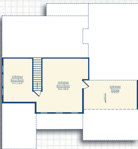
Optional Unfinished Bonus Room Elevation D
