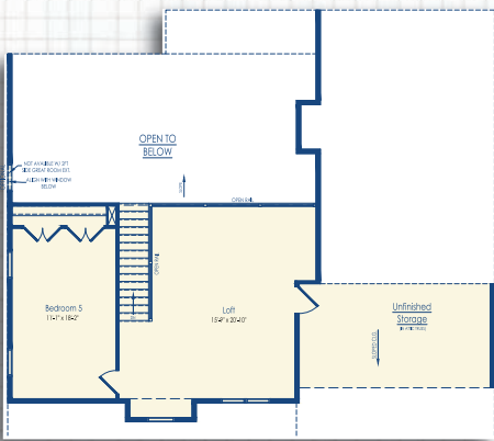
Optional Loft with Bedroom 5 Elevation C
