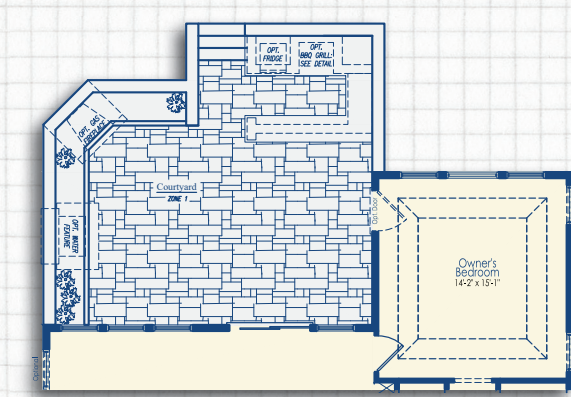
Optional Courtyard with Optional Peninsula Bar
