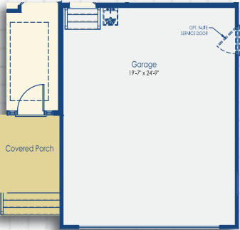
Optional 4’ Garage Extension
