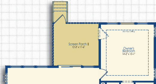
Optional Screen Porch II
