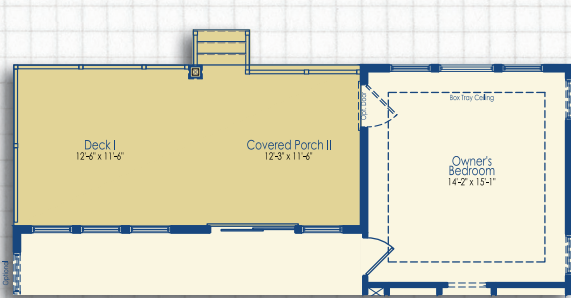
Optional Deck I & Covered Porch II
