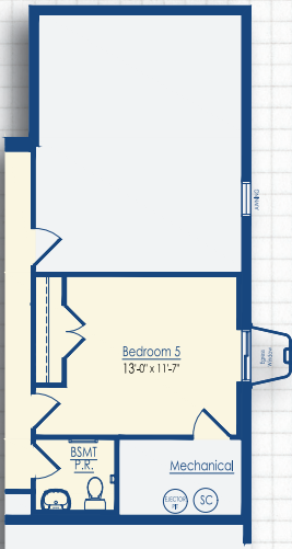
Optional Bedroom 5 with Basement Powder Room
