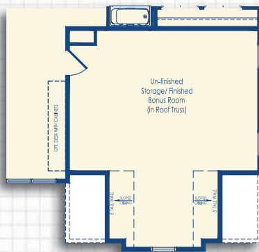
Included Unfinished or Optional Finished Bonus Room with 4' Garage Extension Schell Style D
