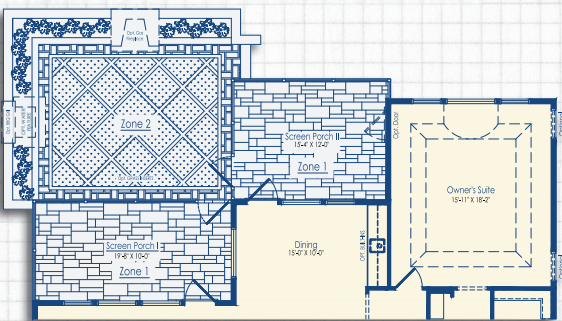
Optional Courtyard with Screen Porch I and Screen Porch II
