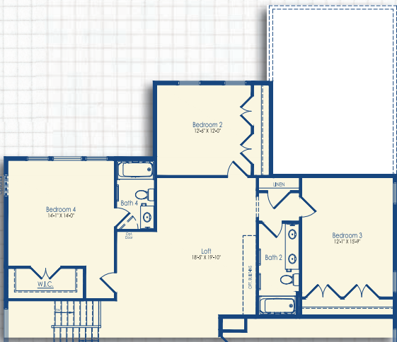
Optional Bedroom 4 with 2' Full Rear Extension Second Floor
