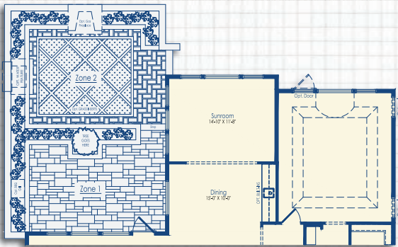
Optional Courtyard with Sunroom I
