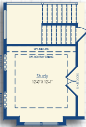
Optional Study Schell Style C
