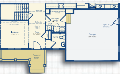
First Floor Optional Schell Style B
