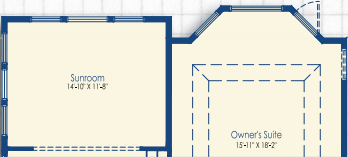
Optional Sunroom with Optional Sitting Area
