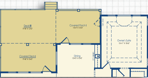
Optional Covered Porch I with Covered Deck I with Decks III and IV *Only available with Extended Loft or Bedroom 4 with Deck IV
