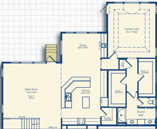
Optional 2’ Full Rear Extension with 2’ Great Room Side Extension
