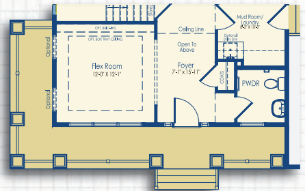
Optional Wrap Around Porch Optional Craftsman Style
