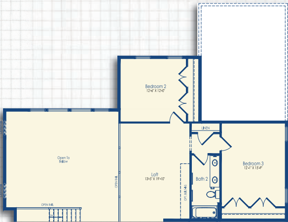
Optional 2' Full Rear Extension and 2' Great Room Side Extension Second Floor
