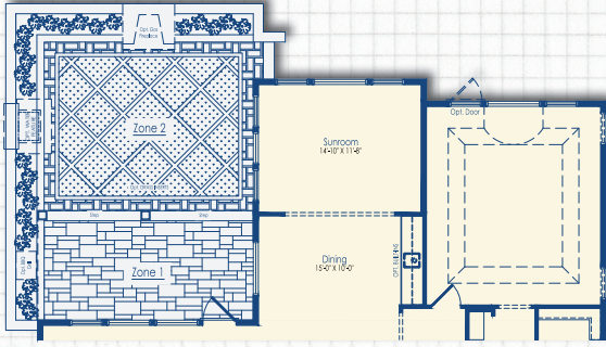
Optional Courtyard with Sunroom I and Deck IV Above
