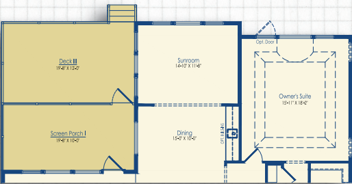
Optional Sunroom I and Screen Porch I with Decks III and IV Above *Only available with Extended Loft or Bedroom 4 with Deck IV
