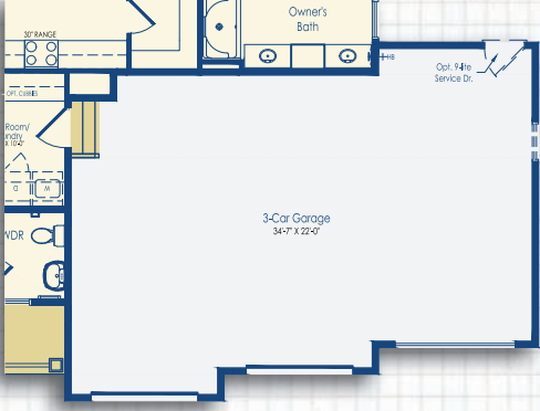
Optional 3-Car Garage Schell Style C
