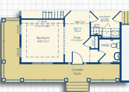
Optional Wrap Around Porch Optional Schell Style A
