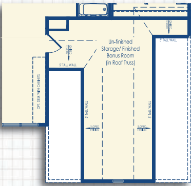
Included Unfinished or Optional Finished Bonus Room with 4' Garage Extension Schell Style B
