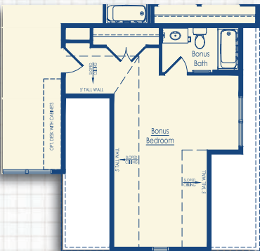
Optional Bonus Bedroom with 4' Garage Extension Schell Style B
