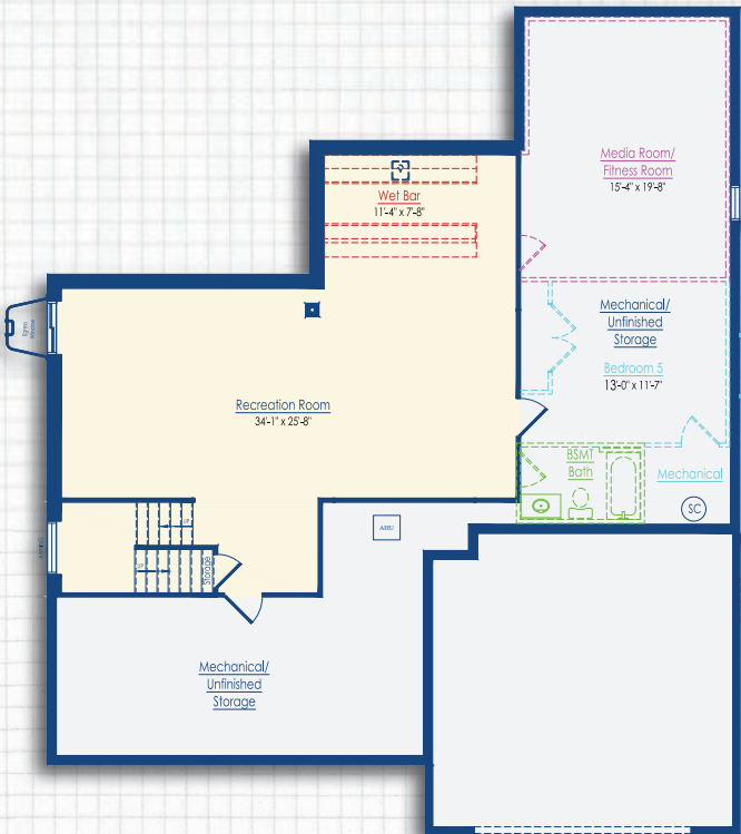
Optional Finished Basement Schell Style A, B, D and Craftsman Style
