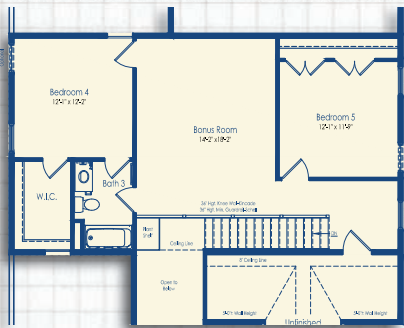
Optional Bonus Room with Bedrooms 4 & 5 and Bath 3
