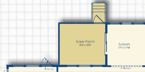
Optional Sunroom with Screen Porch I
