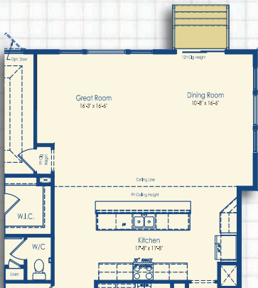
Optional 2' Side Extension
