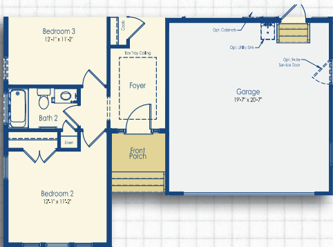
Optional Craftsman Elevation First Floor
