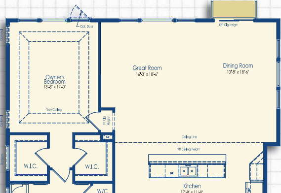
Optional 2' Side Extension and 2' Rear Extension
