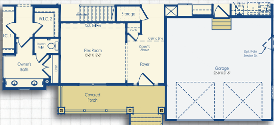
Optional Elevation C First Floor
