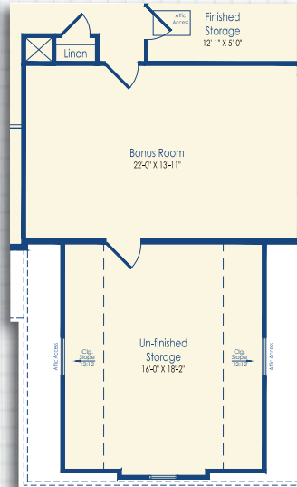
Optional Finished Bonus Room with Unfinished Storage and Optional 3-Car Side-Load Garage Elevation D
