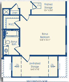
Optional Bonus Bedroom with Unfinished Storage Elevation A *Also available with Optional 4' Garage Extension.
