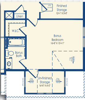
Optional Bonus Bedroom with Unfinished Storage Elevation B *Also available with Optional 4' Garage Extension.
