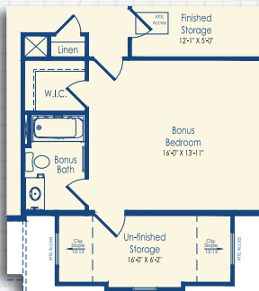
Optional Bonus Bedroom with Unfinished Storage Elevation D *Also available with Optional 4' Garage Extension.
