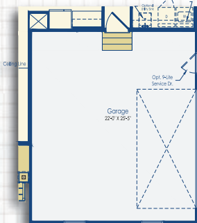
Optional Side-Load Garage with Optional 4' Extension Elevation A & B
