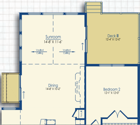
Optional Sunroom with Optional Deck III
