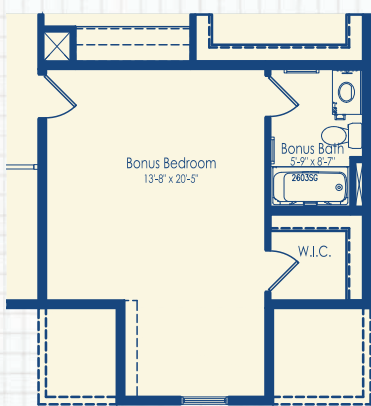
Finished Bonus Bedroom Elevation C
