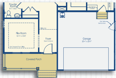
First Floor Elevation B
