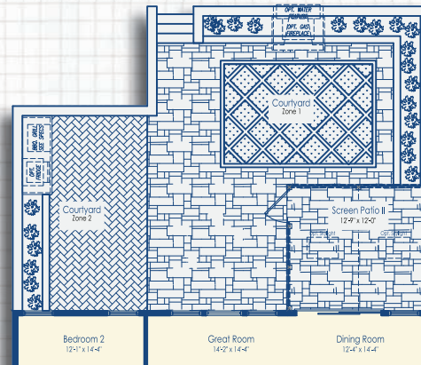
Optional Courtyard with Screen Patio II
