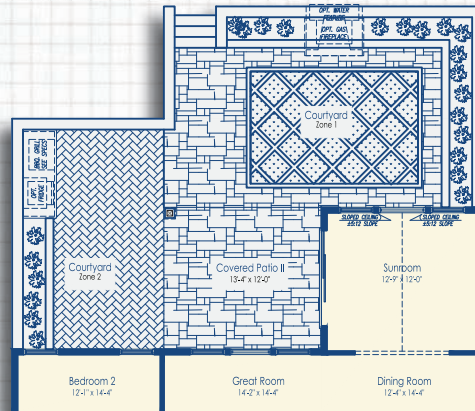
Optional Courtyard with Sunroom and Covered Patio II
