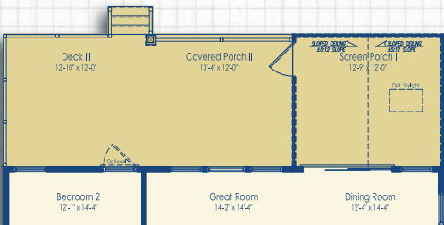
Optional Screen Porch I with Covered Porch II & Deck III
