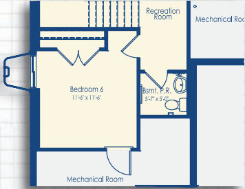
Optional Bedroom 6 with Basement Powder
