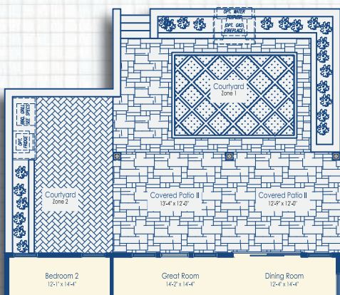
Optional Courtyard with Covered Patio I & II
