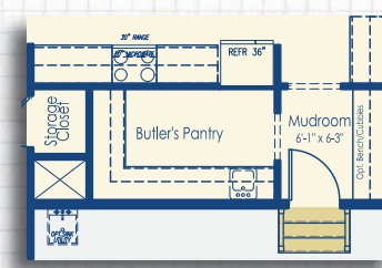
Optional Butler's Pantry
