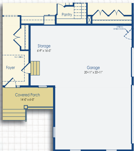
Optional 3-Car Side Load Garage Elevation A & B
