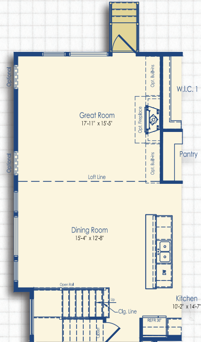
Optional Dining Extension with Great Room Extension
