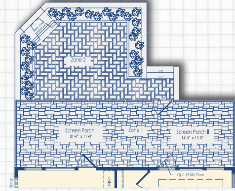
Optional Courtyard with Screen Porch I & II
