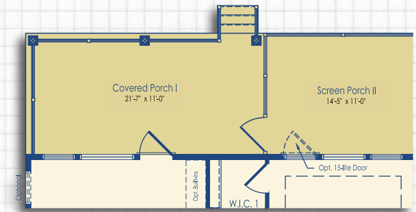
Optional Covered Porch I and Screen Porch II
