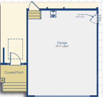
Optional 4' Garage Extension Elevation C
