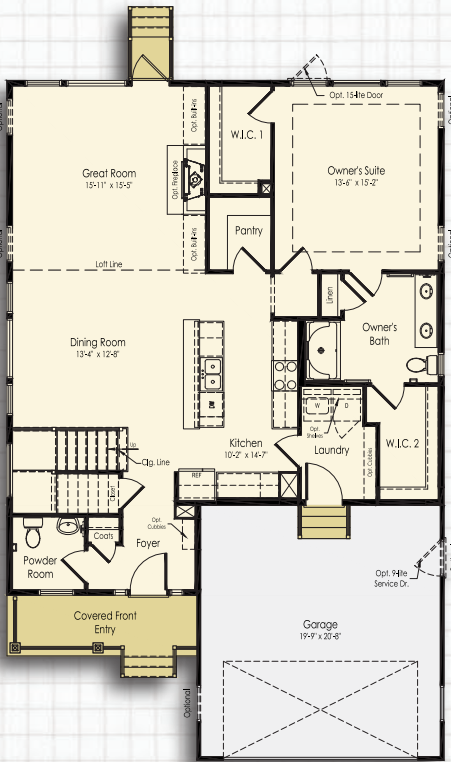
First Floor Elevation B, C, & Craftsman
