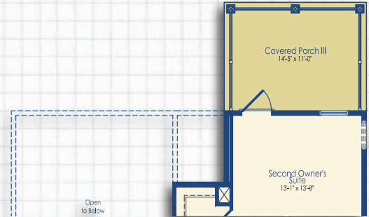
Optional Second Floor Owner's Suite with Covered Porch II and III
