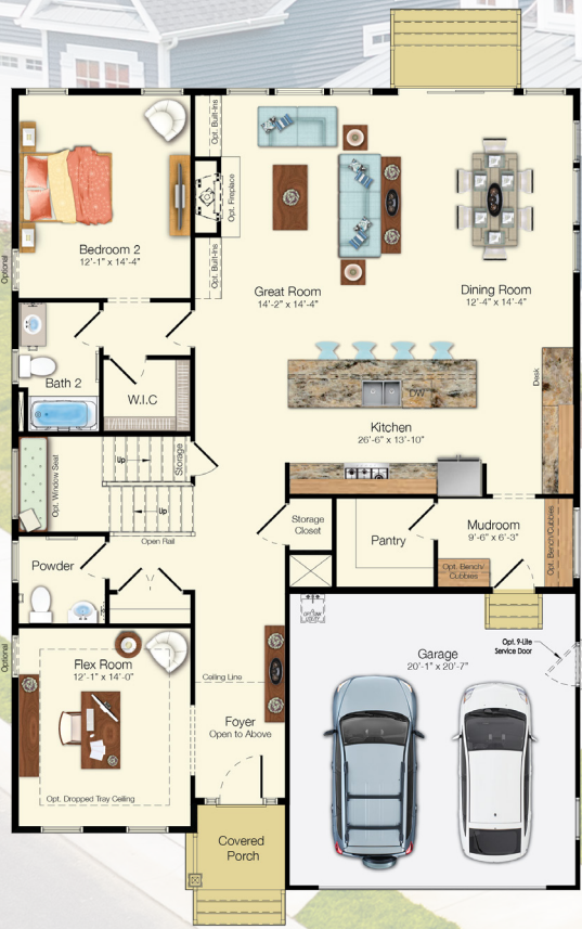
First Floor Elevation A
