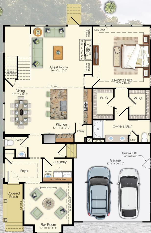
FIRST FLOOR Included Elevation A
